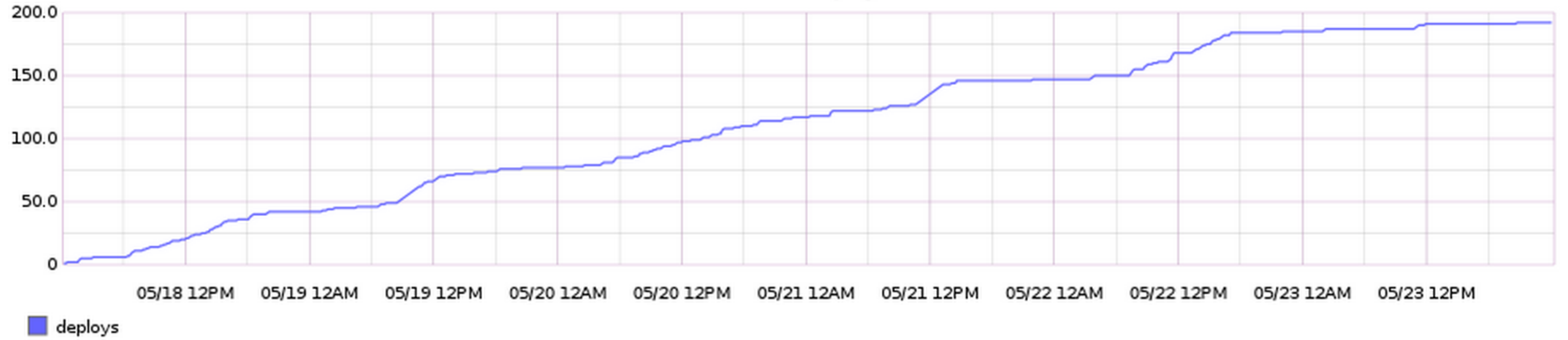
GitHub.com Deploys
